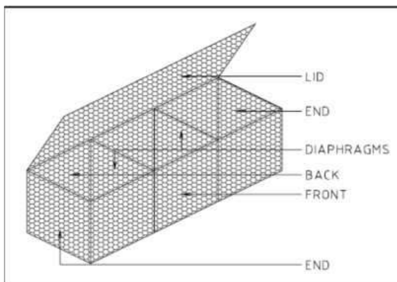
Fig. 24.2 Gabion Box
