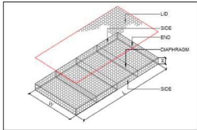
Fig. 24.3 Reno Mattress
