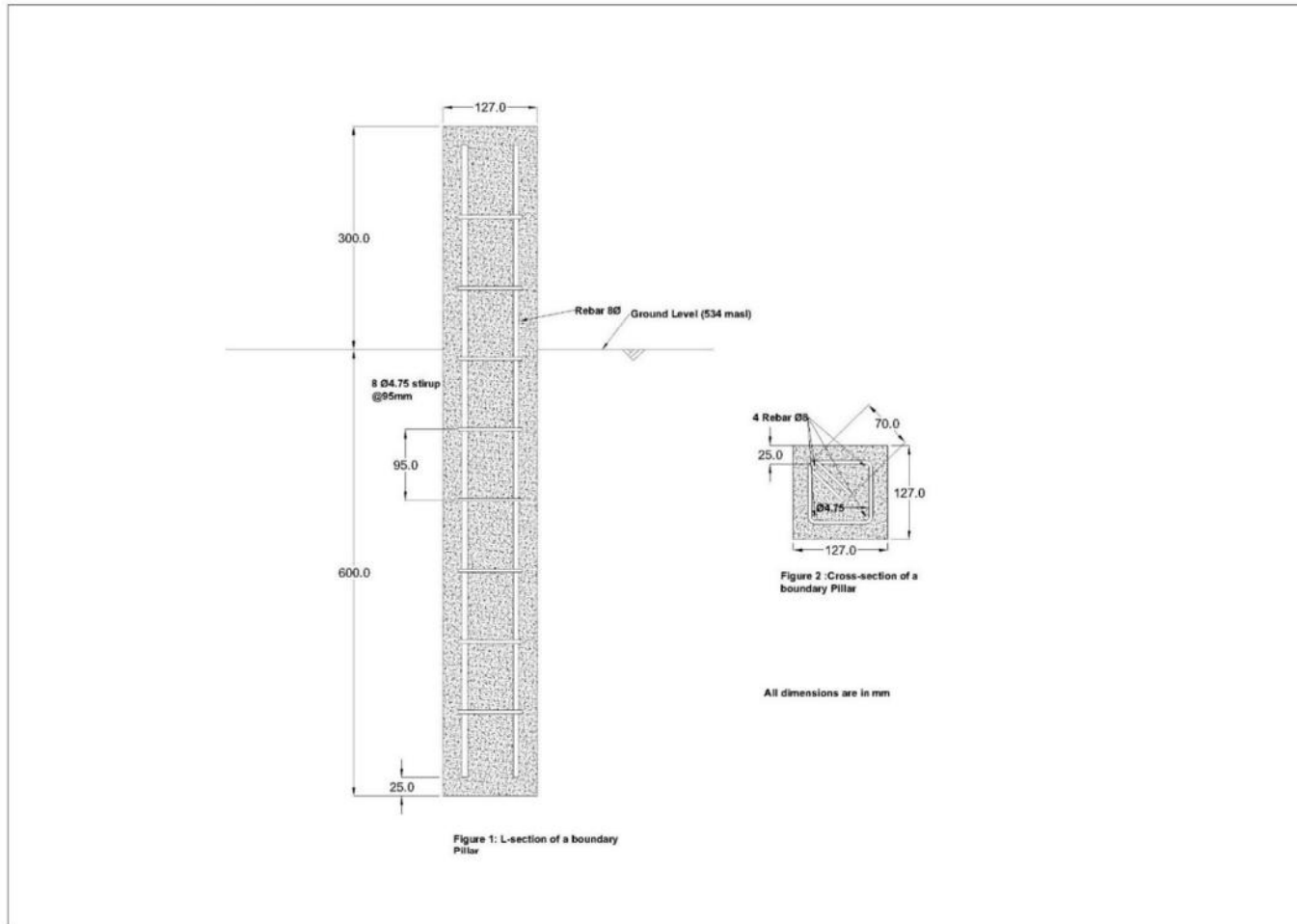
Figure 4 Drawings of boundary pillars
