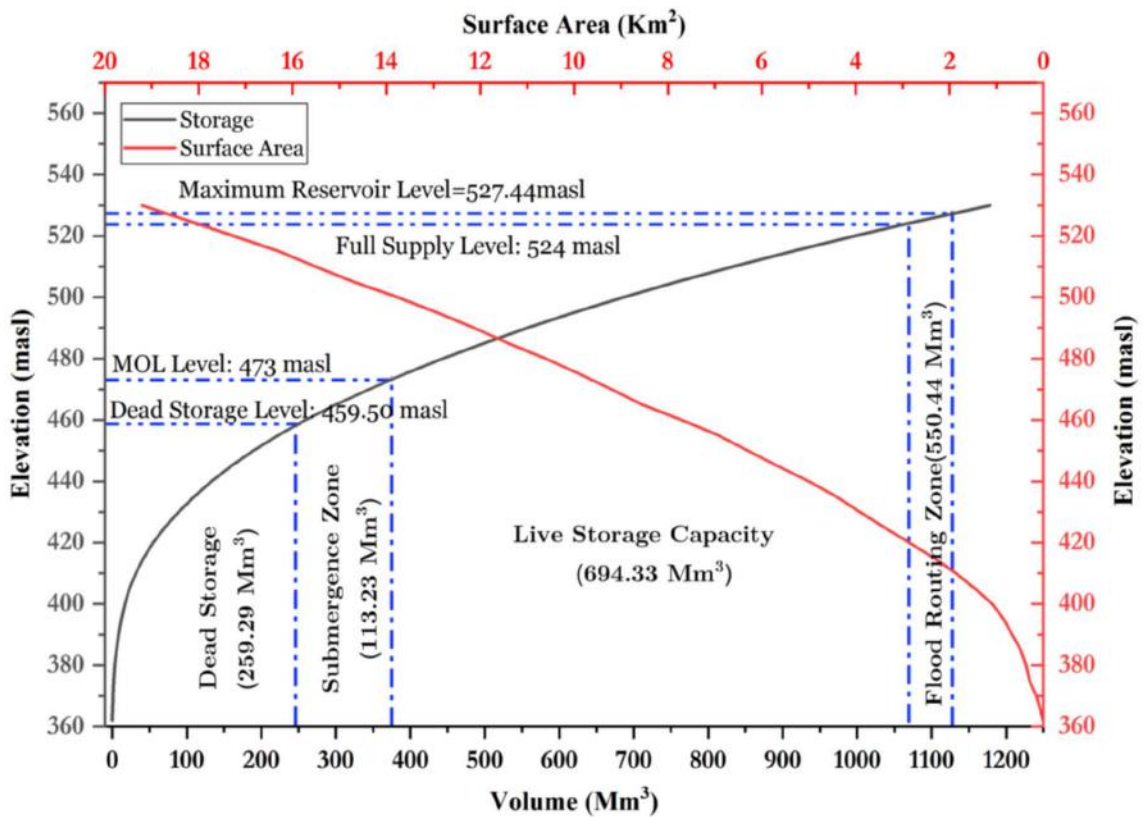
Figure 3 Reservoir characteristics of Naumure Hydro Scheme
