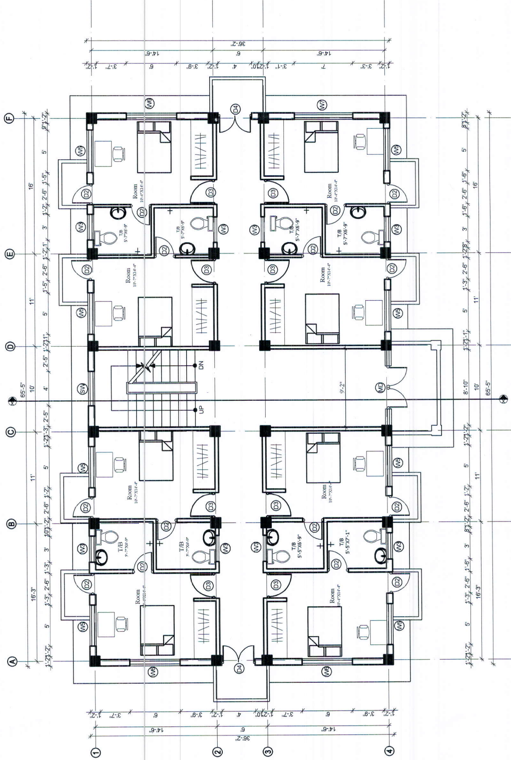
FIRST FLOOR PLAN Floor Area- 2428.96 Sq.Ft.
