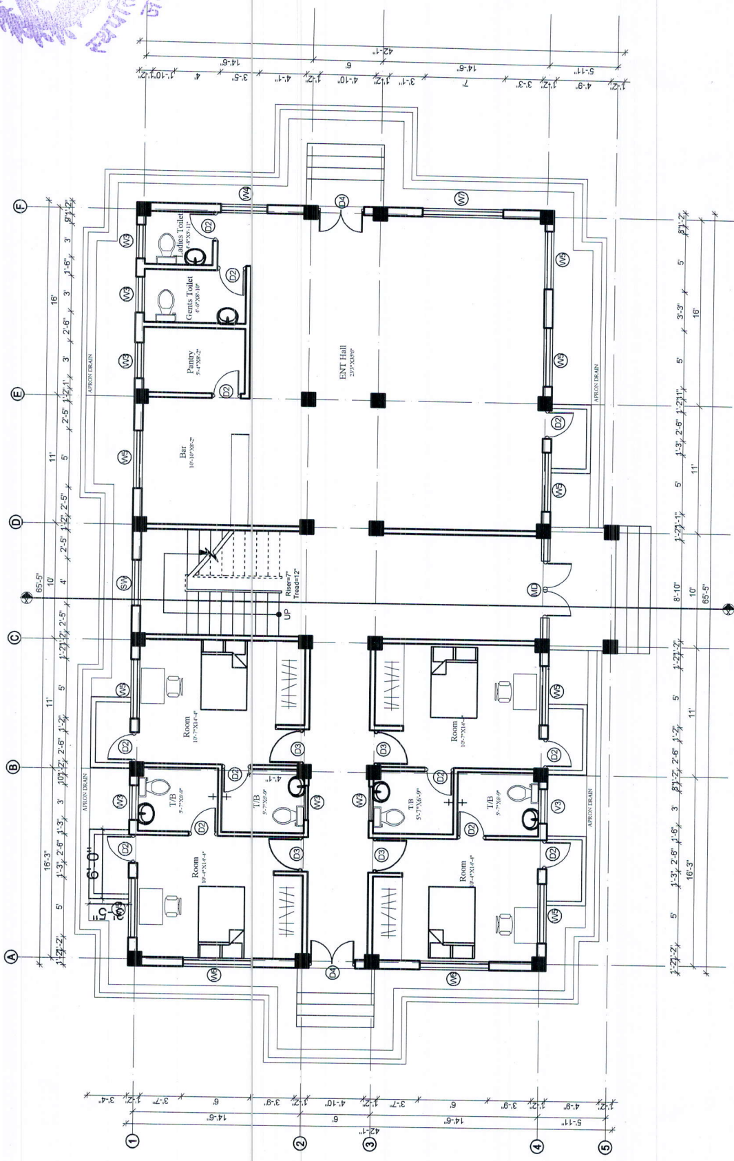
GROUND FLOOR PLAN Ground Coverage - 2324.60 Sq. Ft. Ground Floor Area - 2362.89 Sq. Ft.
